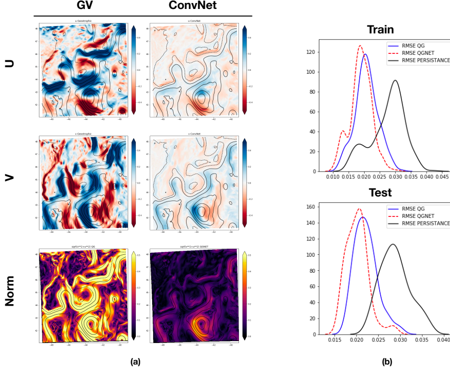
Figure 2: a) An example of the Geostrophic velocities, their norm and the nonlinear additive components produced by the trained ConvNet. SSH contours are shown in black. b) RMSE distributions on the train and test datasets
