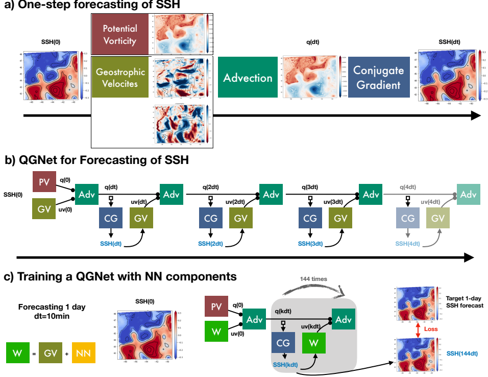
Figure 1: a) 1-step integration of QG equations; b,c) use cases of QG-Net
