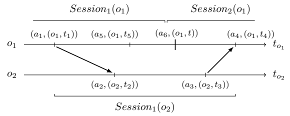
Fig. 4. Contextual action causal dependency in different sessions.
