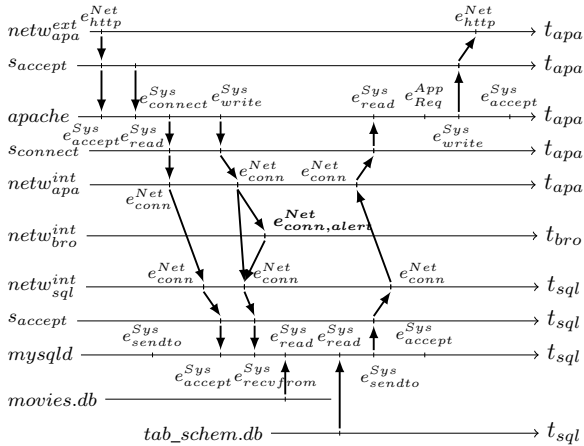
Fig. 2. Visualization of logged events, alerts, and information flows on a space-time diagram.
