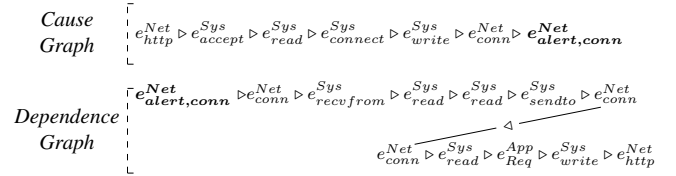
Fig. 11. Cause and dependence graphs of NIDS alert.
