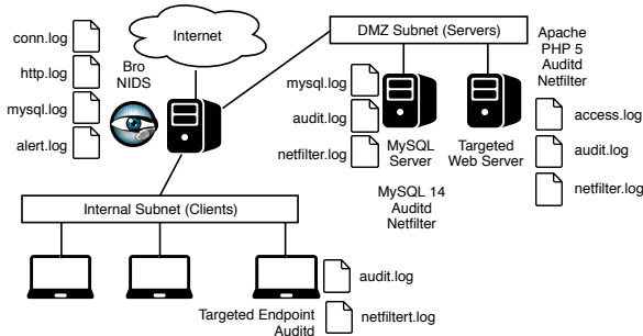
Fig. 12. Network architecture of test environment.
