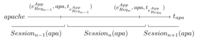
Fig. 6. Apache application contextual event computed from access.log.
