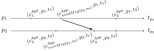
Fig. 7. Message exchange between two applications.
