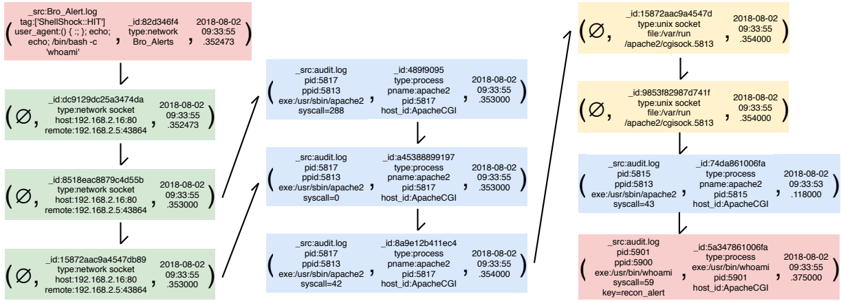
Fig. 13. Contextual event cause graph of whoami alert.
