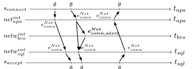
Fig. 9. Network contextual events computed from netfilter and Bro logs.
