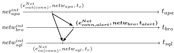
Fig. 10. Message exchange among network objects.
