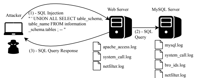
Fig. 1. SQL injection attack scenario on a vulnerable web server.
