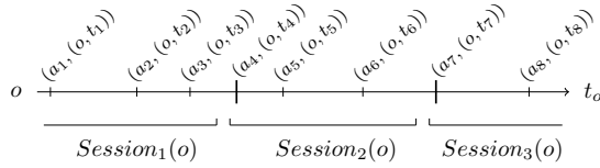
Fig. 3. Sequence of contextual actions and sessions.
