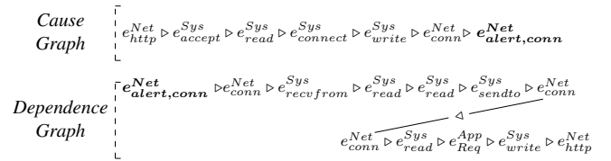
Fig. 11. Cause and dependence graphs of NIDS alert.
