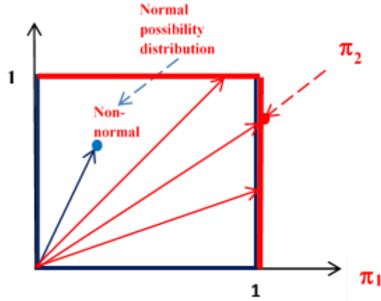
Figure 3. Angle between possibilistic vectors
