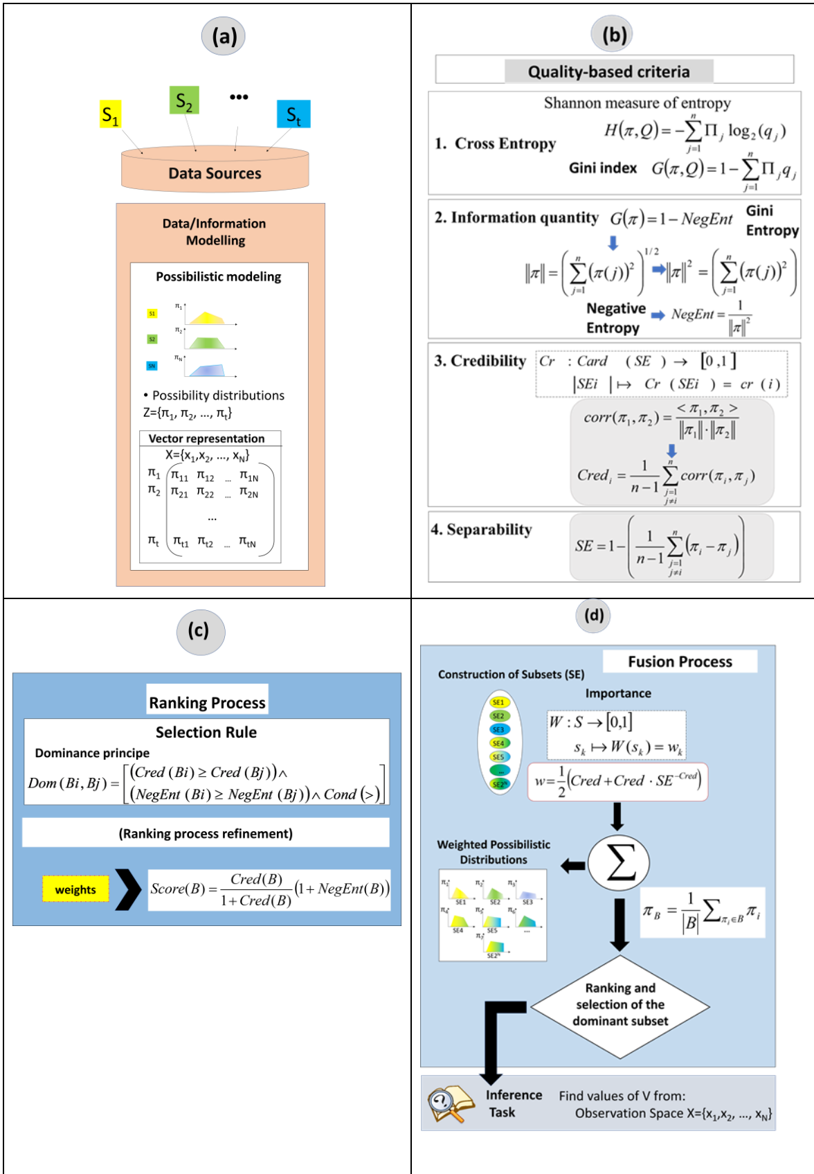
Figure 2. An intelligent quality-based approach for possibilistic sources
