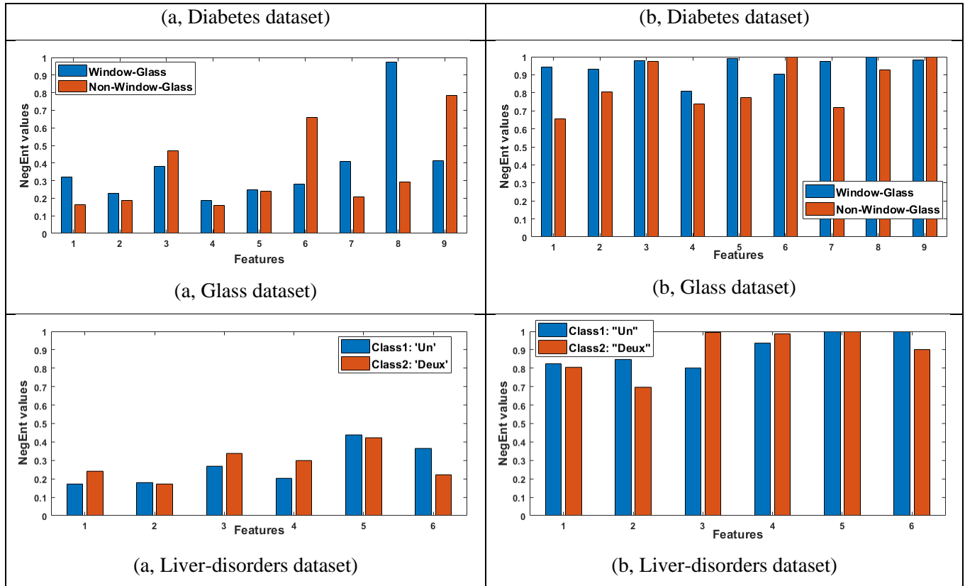
Figure 12. Information quantities ( NegEnt ) in (a) probabilistic framework and (b) possibilistic framework
