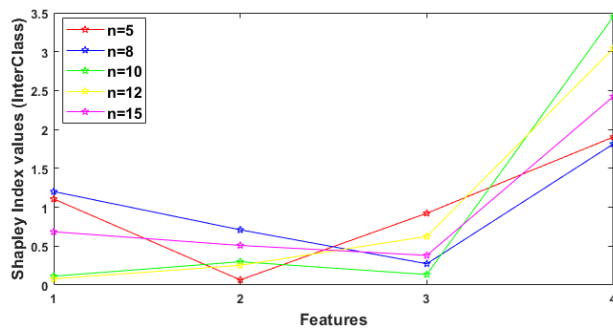
Figure 11. Shapley index values for class discrimination for the Iris dataset for n = 5, 8, 10, 12 and 15
