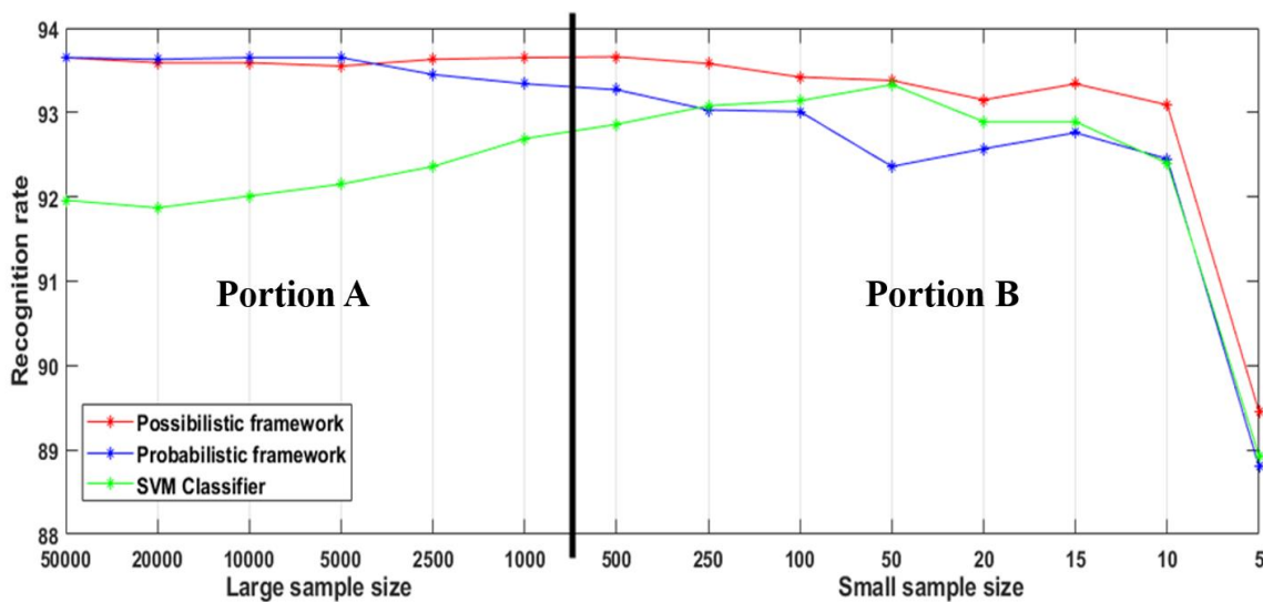
Figure 20. Performance comparison of the possibilistic framework with the probabilistic one and SVM classifier using the large size Skin dataset
