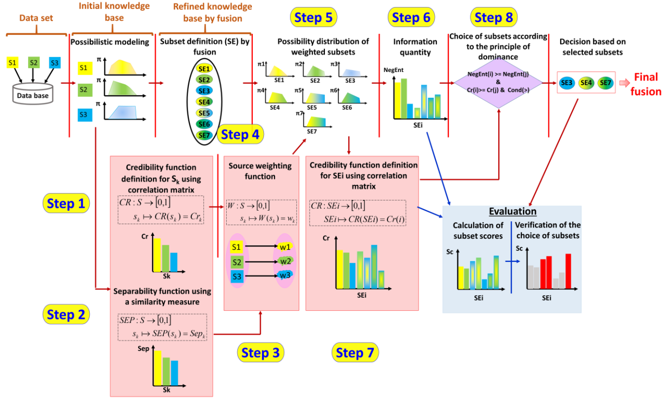
Figure 5. The functional processing (8-step methodology) of the possibilistic approach
