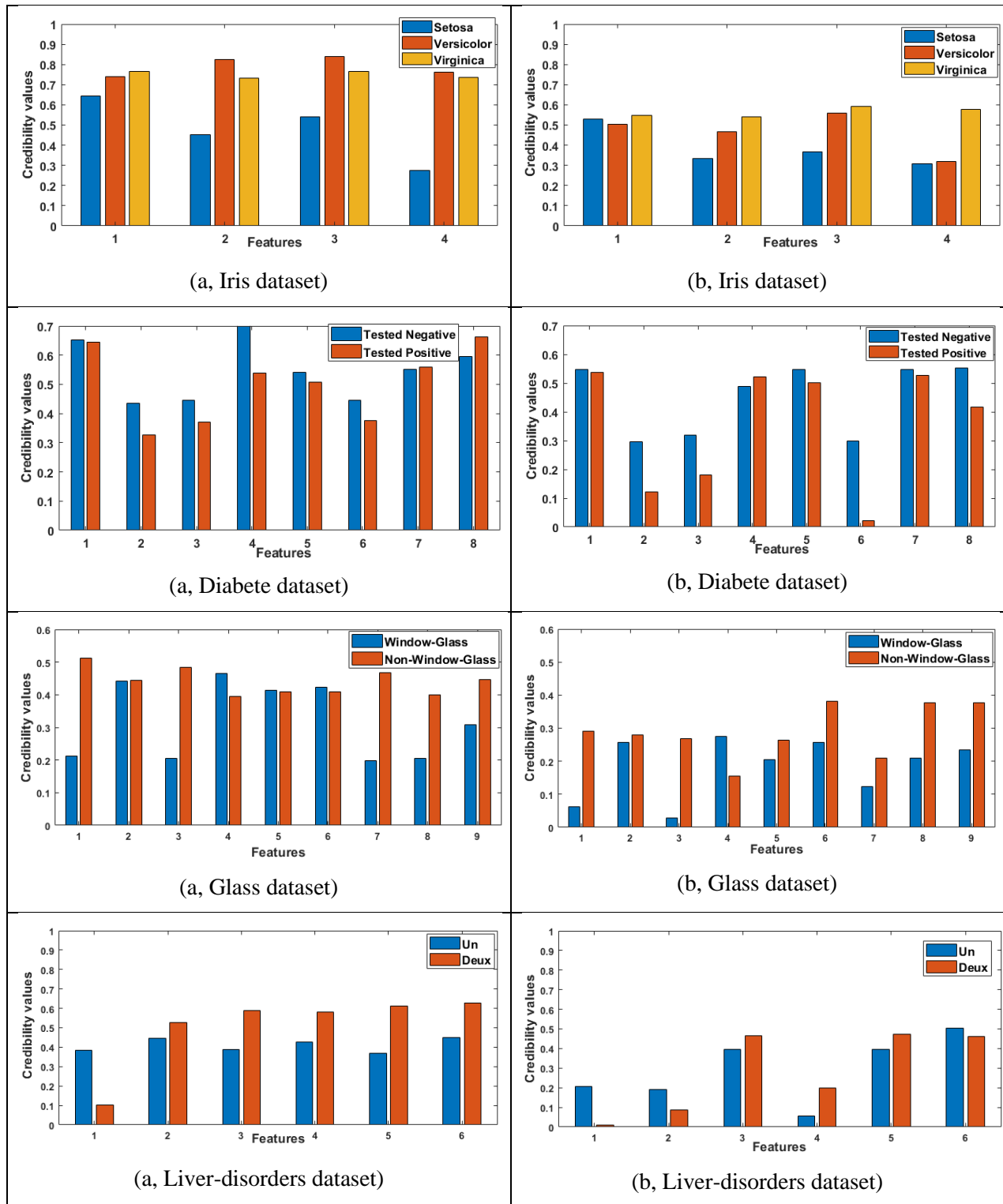
Figure 13. Credibility degrees in (a) probabilistic framework and (b) possibilistic framework
