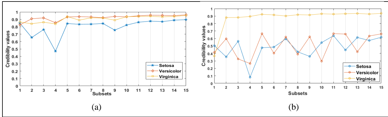
Figure 17. Credibility measures of subsets in (a) probabilistic framework and (b) possibilistic framework for Iris dataset
