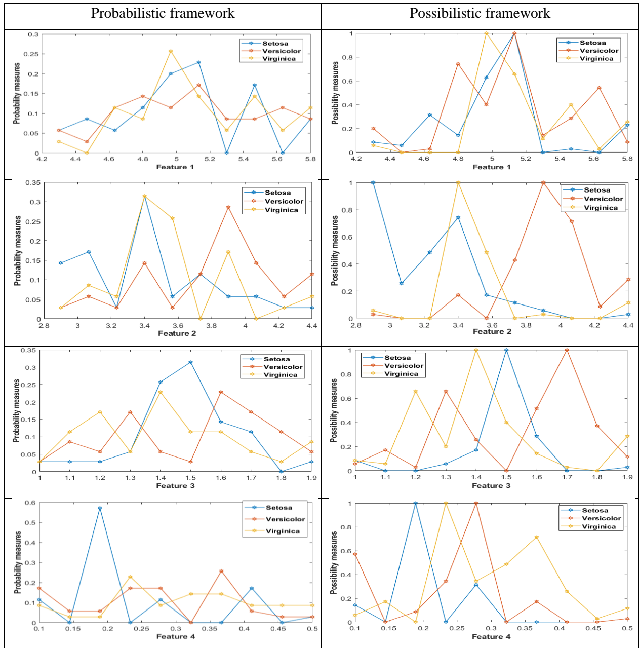
Figure 10. Class representations in probabilistic and possibilistic frameworks using the Iris dataset
