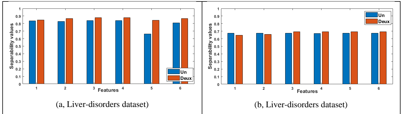
Figure 14. Separability degrees in (a) probabilistic framework and (b) possibilistic framework
