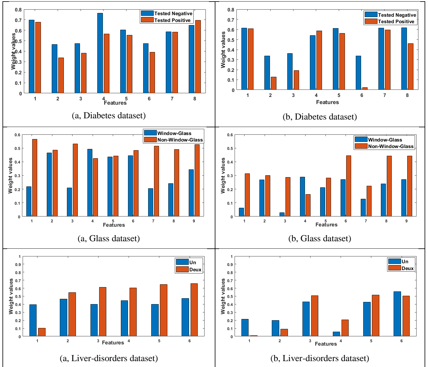
Figure 15. Weight degrees in (a) probabilistic framework and (b) possibilistic framework
