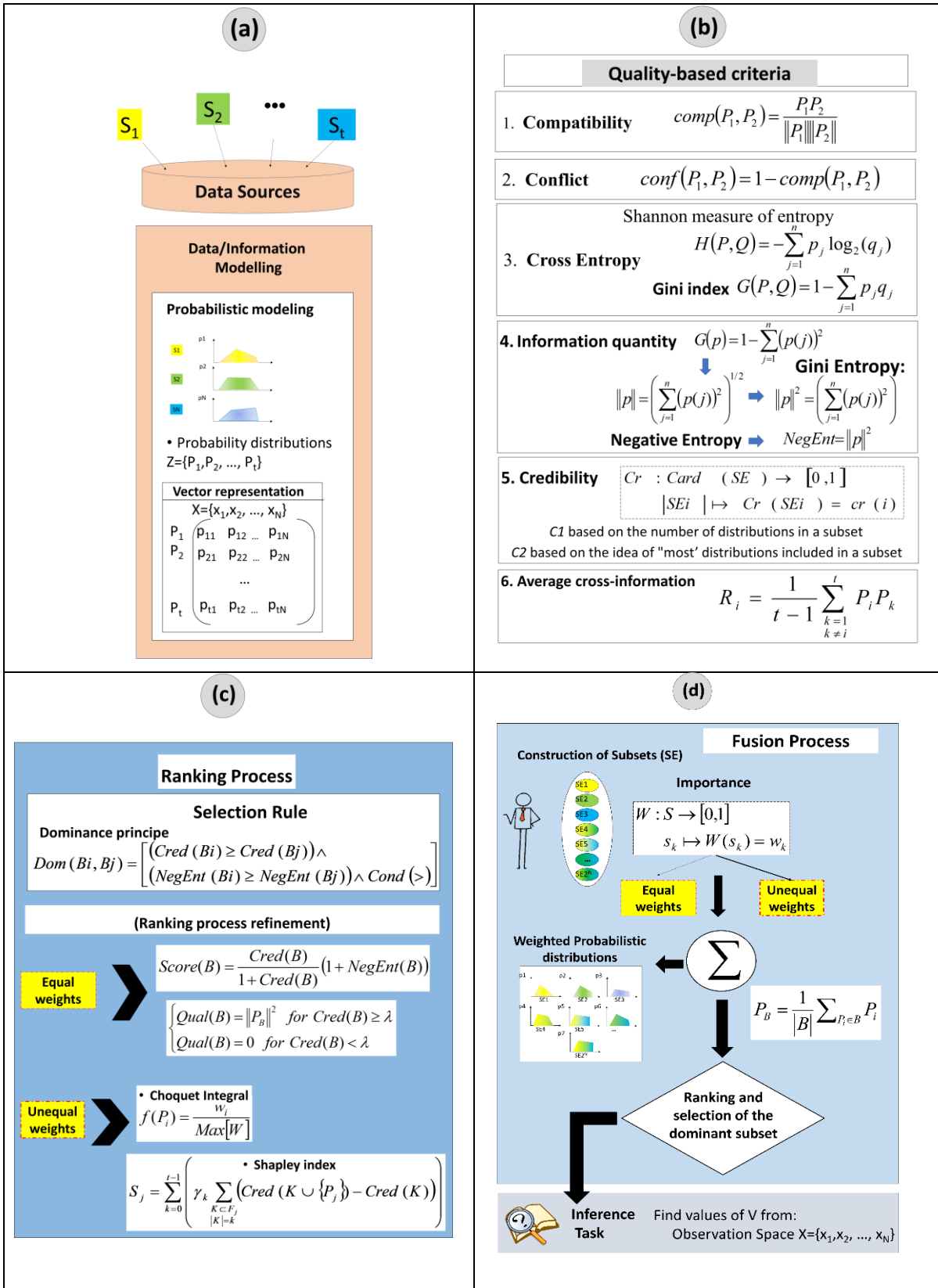
Figure 1. Intelligent quality-based approach of Yager & Petry for probabilistic sources
