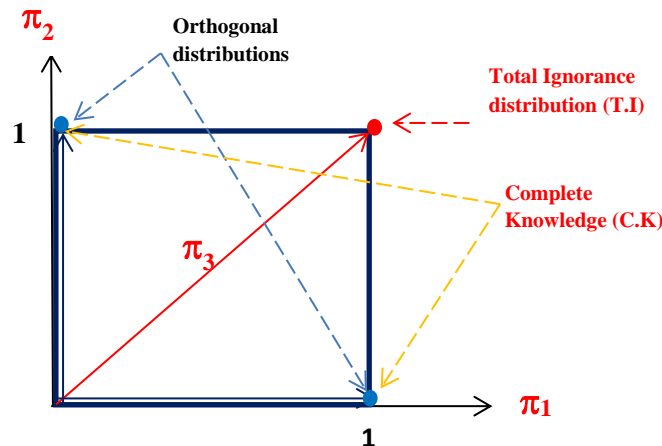
Figure 4. Illustration of orthogonal, complete knowledge and the total ignorance distributions
