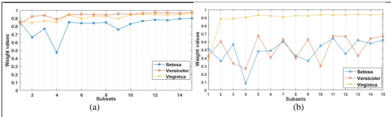
Figure 18. Weight values of subsets in (a) probabilistic framework and (b) possibilistic framework for Iris dataset
