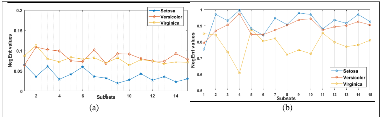
Figure 16. Information quantity ( NegEnt ) of subsets in (a) probabilistic framework and (b) possibilistic framework for Iris dataset
