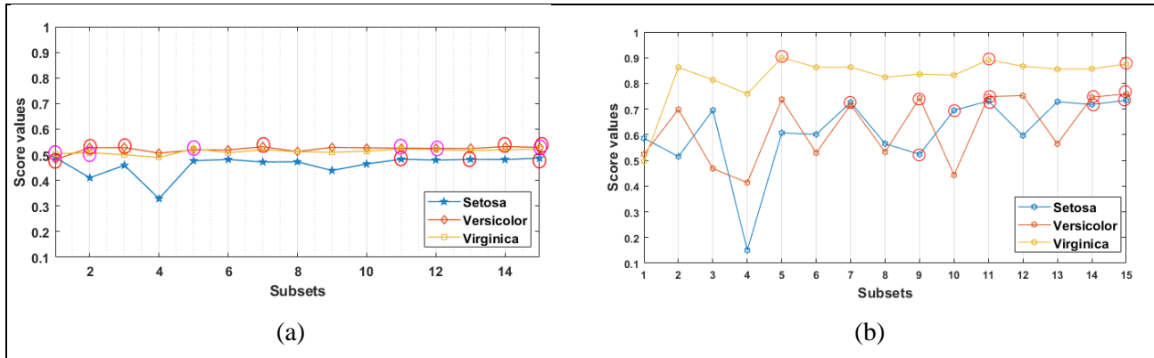
Figure 19. Scores of subsets in (a) probabilistic framework and (b) possibilistic framework for Iris dataset
