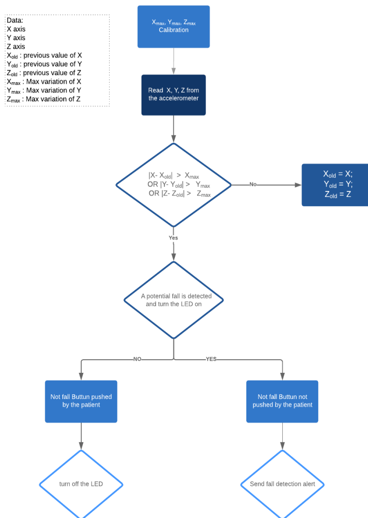
Figure 5. Simple fall detection algorithm using an accelerometer.
