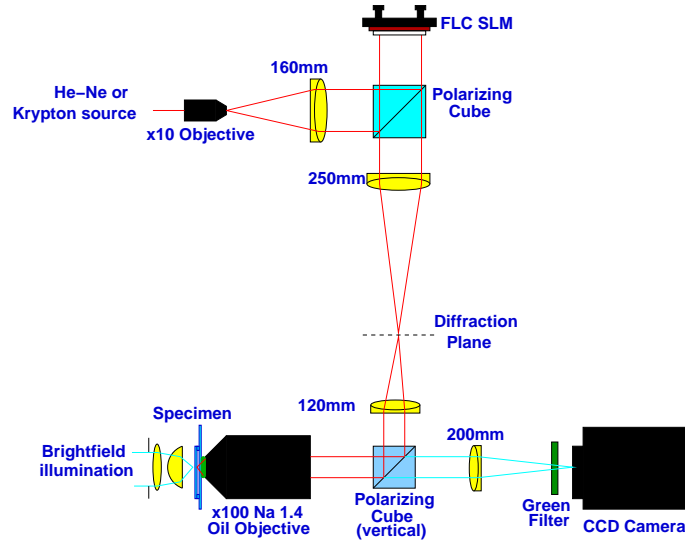
Fig. 1. Schematic layout of optical system
