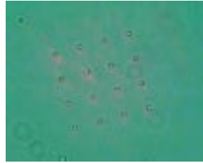
Fig. 2. 4 \times 4 array of traps on 5\ \mu\text{m} pitch with 700 mW total input power. Movie of capture of final trap available at: http://www.cosmic.ed.ac.uk/movies/tweezers/holographic/4x4array.avi
