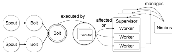
Fig. 8: Storm architecture
