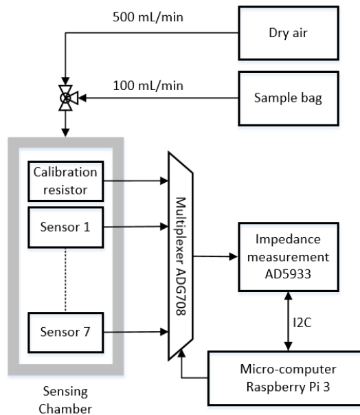
Figure 1: Schematic of the proposed electronic nose system
