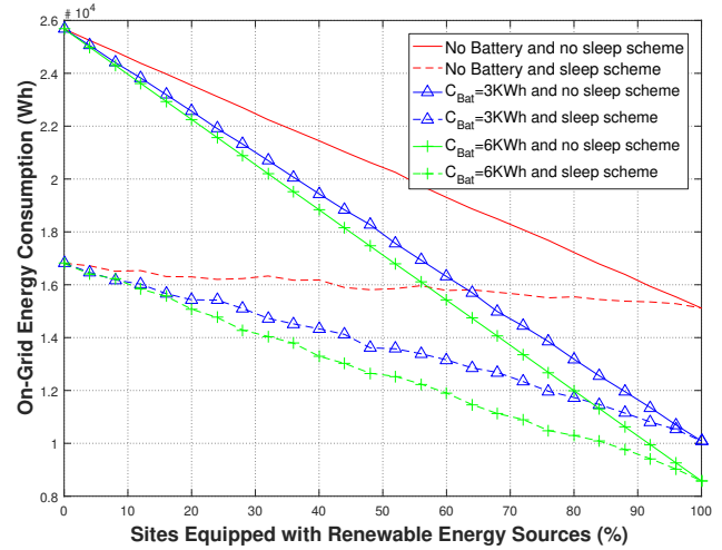
Fig. 3: Network energy consumption over one day, with a 12.5m 2 solar panel surface area.
