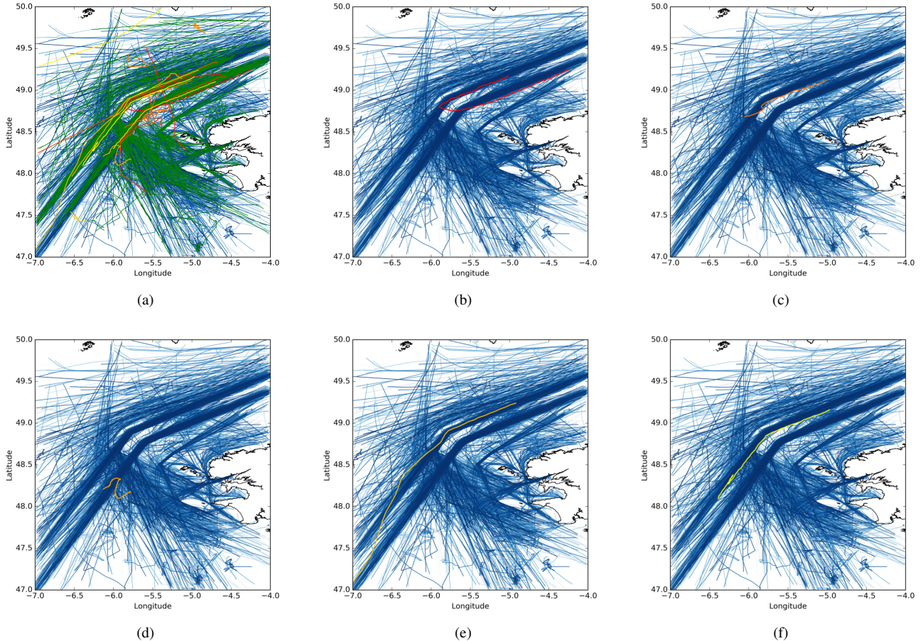
Fig. 7. Abnormal tracks detected by the proposed a contrario model (Ushant dataset). (a) All tracks detected in the test set; blue: tracks in the training set; green: normal tracks in the test set; other colors: abnormal tracks in the test set. (b) Abnormal U-turn. (c-d) Divergences from maritime route. (e) Abnormal route change. (f) Abnormal double-U-turn.
