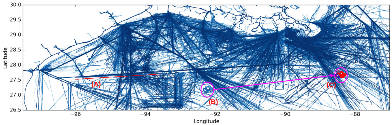
Fig. 5. Example of the a contrario anomaly detection on simulated dataset (Gulf of Mexico dataset). The circle-shaped tracks in zones (C) are simulated by translating from (B); (A) is a detection of a divergence from maritime route.
