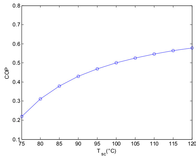
Figure 5. Solar concentrator temperature effect on the Coefficient of Performance for ( T_{si} = 28 °C, T_{sf} = 10 °C).
