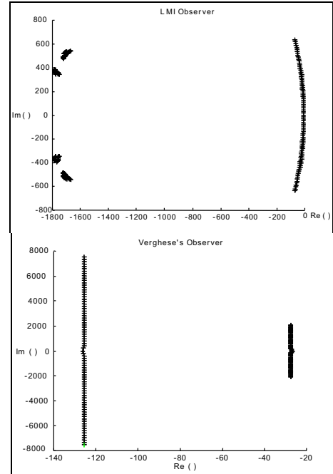
Figure 3: Roots locus
