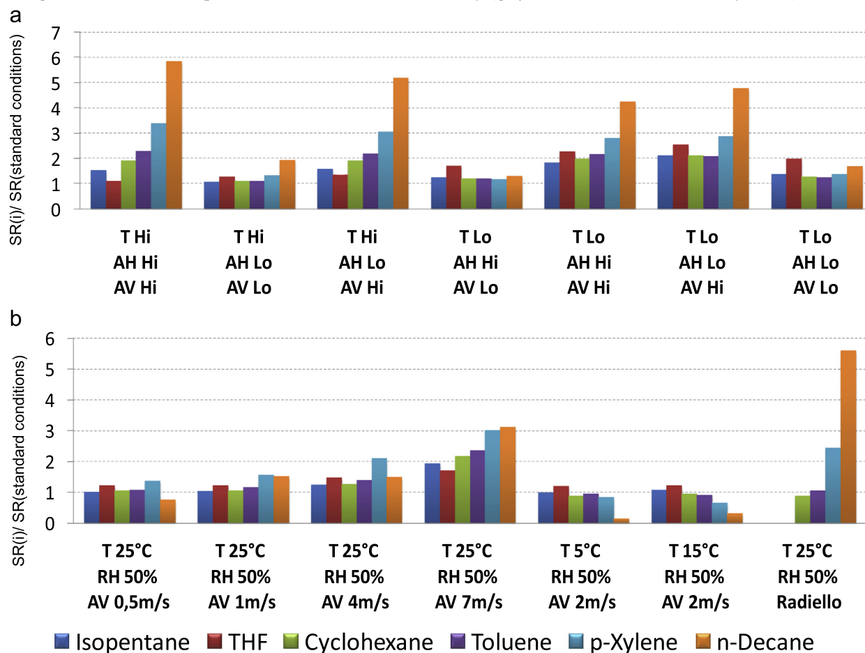
Fig. 1. Sampling rate variations at several weather conditions relatively to a sampling rate determined: under closer standard conditions ( 25^{\circ}\text{C} , 30\% \text{ RH} , 2 \text{ m s}^{-1} ) for the thin diffusive body (a) and under standard conditions ( 25^{\circ}\text{C} , 50\% \text{ RH} , 2 \text{ m s}^{-1} ) for the thick diffusive body (b). Hi: High; Lo: Low; T: temperature ( ^{\circ}\text{C} ), H: absolute humidity ( \text{g of water m}^{-3} ), AV: air velocity ( \text{m s}^{-1} ).
