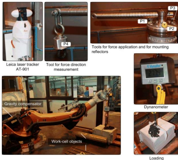
Figure 2. Experimental setup for manipulator elastostatic calibration
