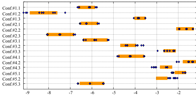
Figure 5. Distributions of the manipulator end-effector deflections along Z directions: ♦ - experimental data; — - computed
