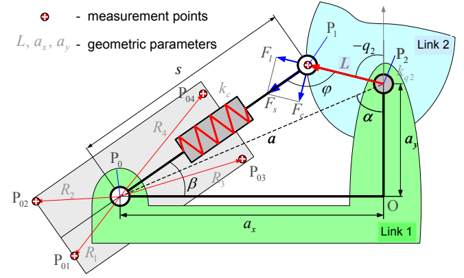
Figure 3. Gravity compensator model
