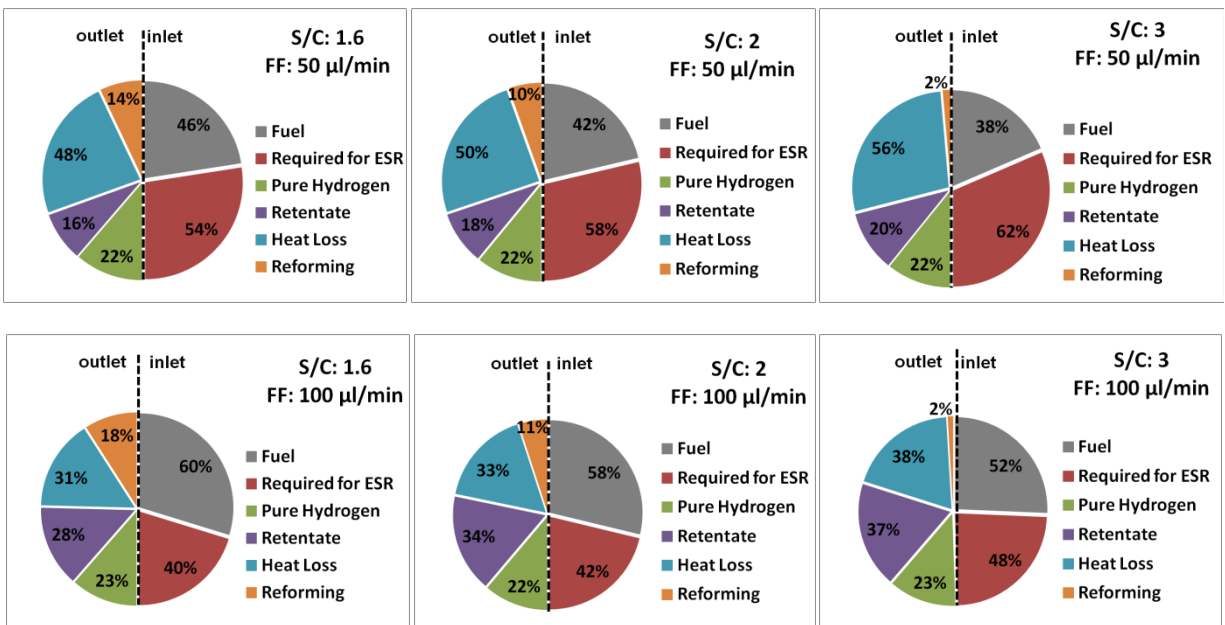
Fig. 11: Exergy flows at 923 K and 12 bar at various S/C ratios. FF represents the fuel flow rate in μl/min.
