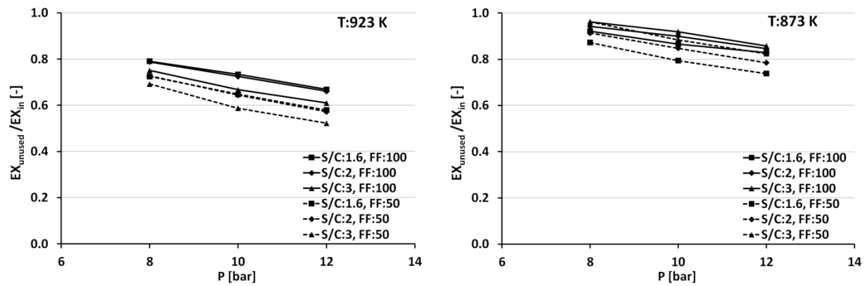
Fig. 14: Unused exergy for the insulated reactor. FF represents the fuel flow rate in \mu\text{l}/\text{min} .
