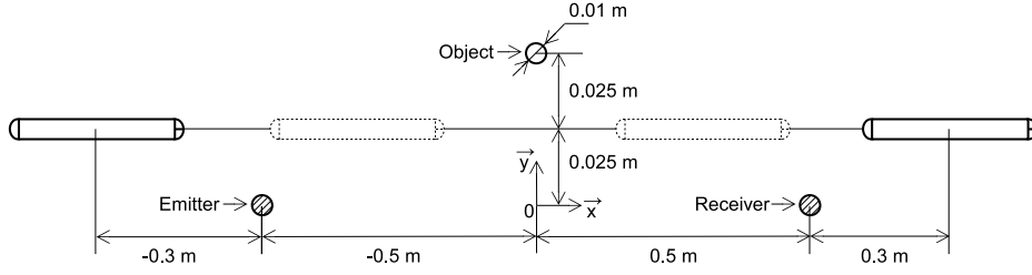
Figure 7: A passive electric probe is translated between two external electrodes (one emitter and one receiver) in the presence of a small insulating sphere.
