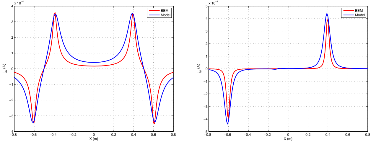
(a) Axial current versus the position of the passive probe along the path.
