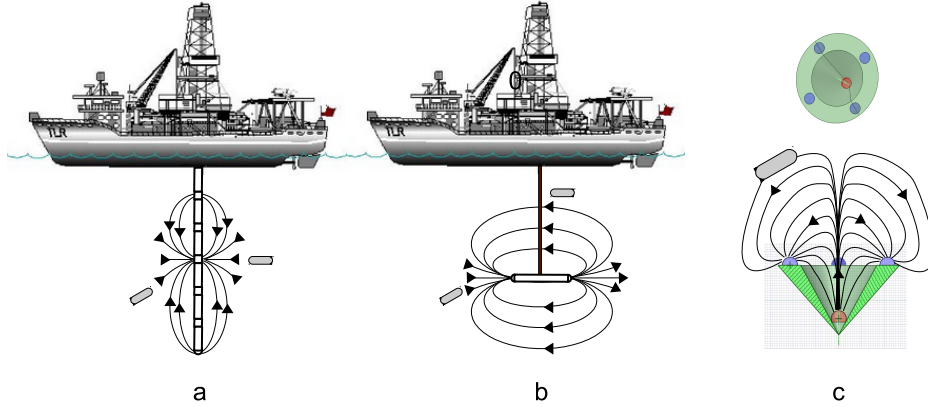
Figure 20: Outline schematic of electric docking stations. (a) An immersed vertical pole on which are arranged a set of electrodes set under controlled voltages in order to attract the AUVs for recharging their batteries. (b) This docking station is directly inspired from the probes design of the article. It could be yaw controlled in order to help docking. (c) An insulating nozzle confines the electric current lines which flow from the emitter (at the top of the cone) to a set of receivers located at the entrance to the nozzle. This field of electric lines could steer an AUV towards the emitter where the docking can be achieved by an anchoring mechanical device.
