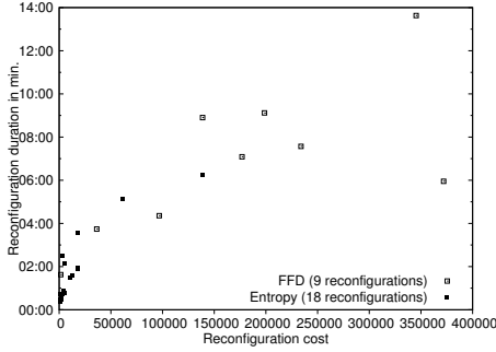
Figure 14. Reconfiguration costs computed by FFD and Entropy
