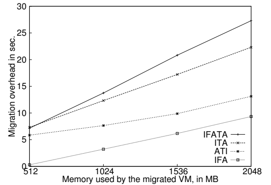
Figure 9. Impact of migration on VM performance
