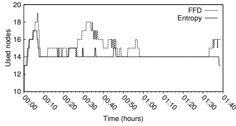
Figure 16. Number of nodes used with FFD and Entropy
